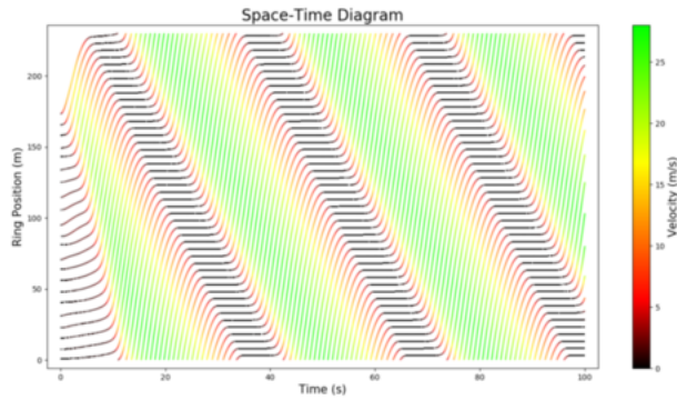
(c) 22 OVM vehicles from a nonuniform ring road initial state, showing stop-and-go traffic with an average speed of 7.8 m/s.
