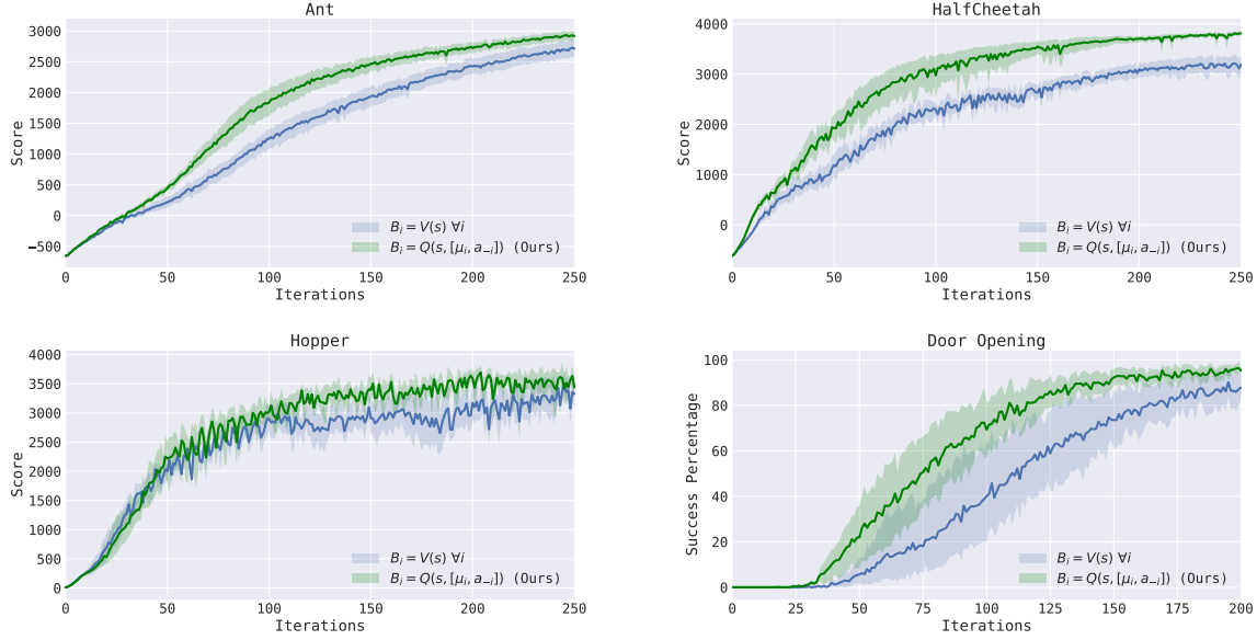
Figure 17: Comparison between value function baseline and action-conditioned baseline on various continuous control tasks. Action-dependent baseline performs consistently better across all the tasks.
