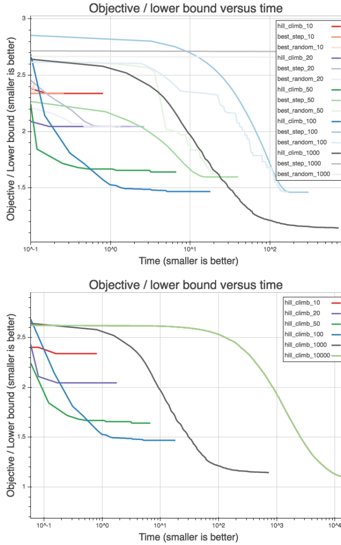
Figure 46: This figure demonstrates the convergence of the methods in the SF Bay Area setting. Top: For the smaller problem instances: \{10, 20\} , the three methods displayed converge to the same ratio to the lower bound, but hill climbing converges much faster and, for the larger problem instances of \{50, 100, 1000\} , to a lower ratio. The classical local search method gives a steady but slow convergence, whereas the random neighborhood search gives a more jagged convergence. In the case of size 50 and 100, the classical local search method converges to a slightly lower ratio than hill climbing, implying that hill climbing may have reached a different local optimum (or not reached one at all). In the case of problem size 1000, the best_step and best_random (the gray near-horizontal lines) are further from the lower bound and were cut short due to the timeout. Bottom: We display convergence only for the hill climbing method and problem instances \leq 100K . In all instances the problem converges to between 1.1 to 2.4 times the lower bound. Notably, in the largest problem size, hill climbing achieves a ratio close to 1, implying that the solution is near optimal. Note that the x-axis is on a log scale.
