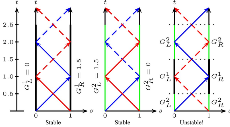
Fig. 1. Instability by switching according to Example 1.
