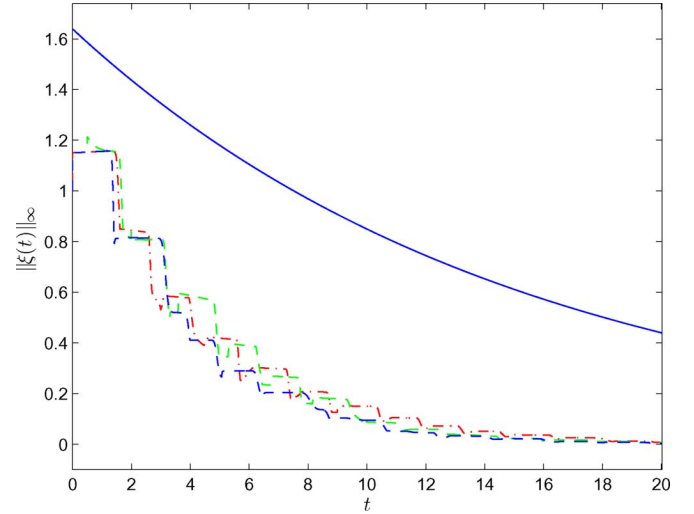
Fig. 4. Exponential bound for \|\xi(t)\|_\infty obtained in Theorem 1 (solid line) and the observed decay for three different switching signals (dashed lines) of solutions for the system considered in Example 2.
