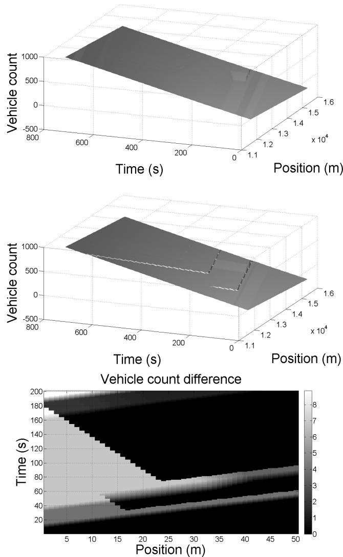
FIG. 6.1. Solutions to data assimilation and data reconciliation problems. Top: The solution to the data reconciliation problem. Middle: The solution to the data assimilation problem involving 50 boundary conditions sampled intervals and 11 internal conditions of the form (6.2). Both solutions were computed simultaneously by solving Problem (5.8) numerically. Bottom: Difference (in number of vehicles) between the solution to the data reconciliation problem and the solution to the data assimilation problem.
